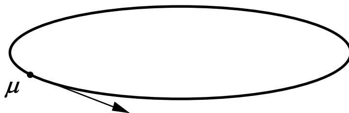
Figure 1. In the CERN storage ring unstable particles ("muons") circulated with a speed smaller than that of light by only six parts over ten thousand. It was observed that muons disintegrated after a lifetime 29,33 times larger than for muons at rest.
